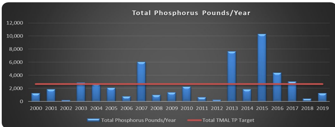
Figure 5 Total Phosphorus Trend
