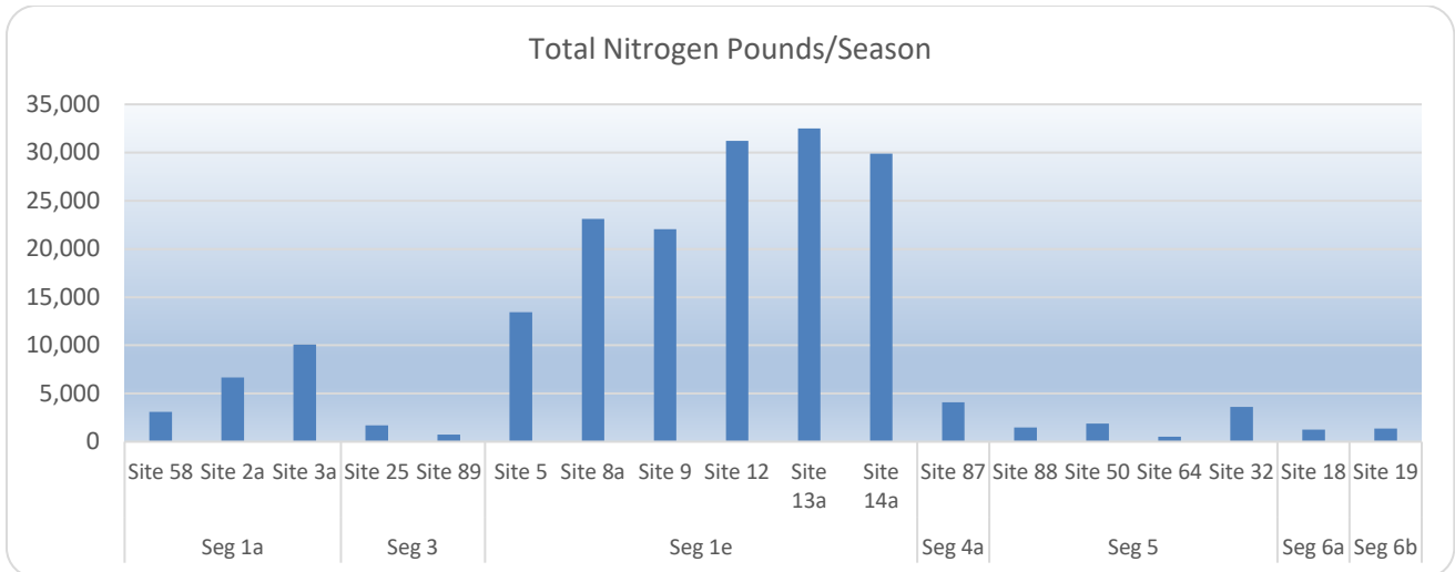
Figure 4 Total Nitrogen Loading by Stream Segment in the Watershed
