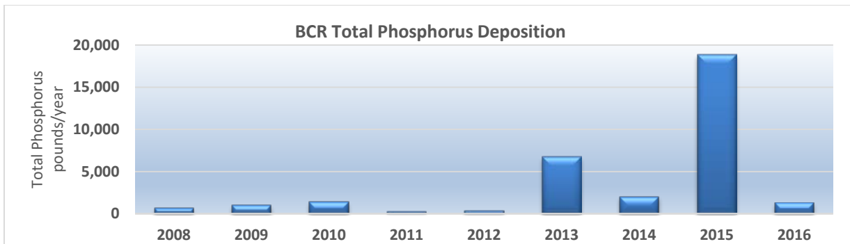
Figure 2 Annual Total Phosphorus Deposition into Bear Creek Reservoir Bottom Sediments
