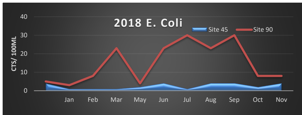
Figure 7 E.coli at Site 45 vs. Site 90 at Wadsworth
