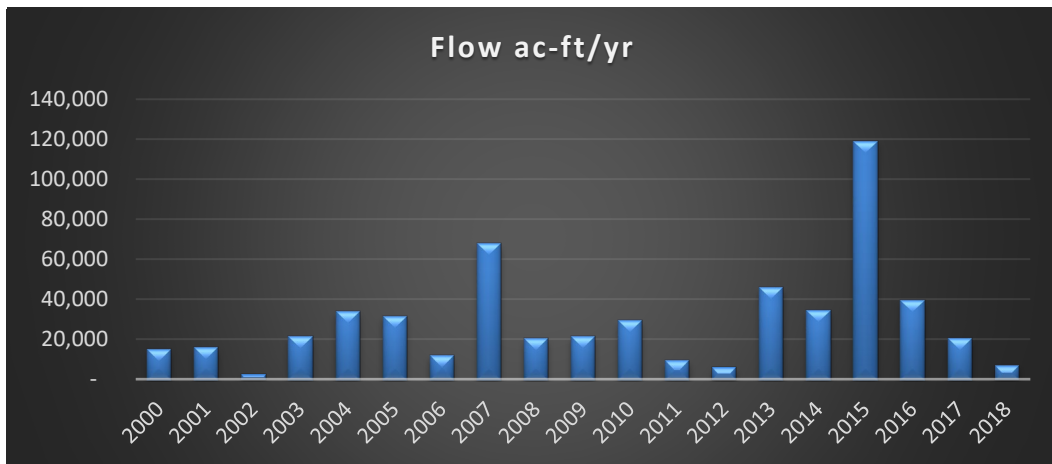
Figure 4 Flow Trend at BCWA Site 45
